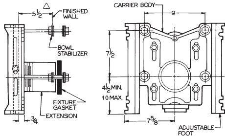
Carrier shown in Siphon Jet Position
