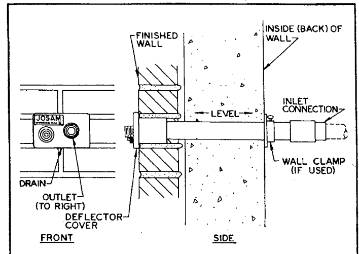
FIGURE 2—HYDRASAN I MODEL 71050 INSTALLATION
