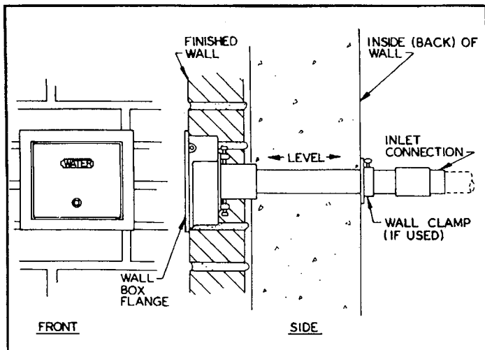
FIGURE 1—HYDRASAN I MODEL 71000 INSTALLATION
