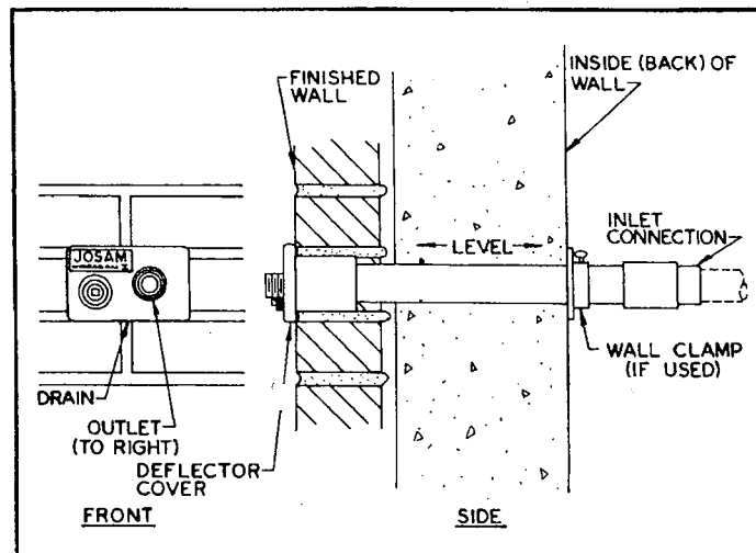
FIGURE 2—HYDRASAN I MODEL 71050 INSTALLATION
