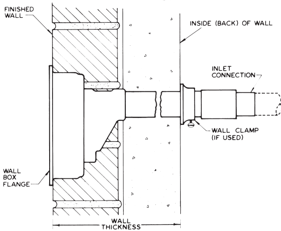
Drawing showing how to determine wall thickness
