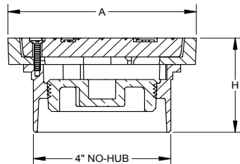
CO-600-NB-SQ SQUARE NIKALOY RIM AND COVER
